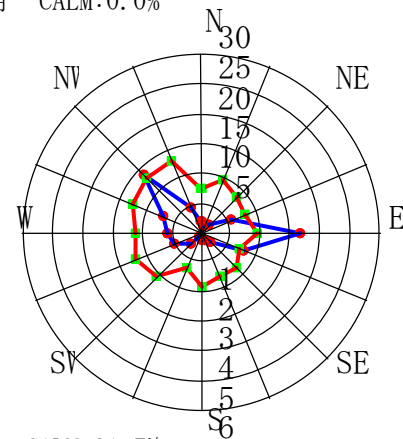
3月 CALM:21.7%
