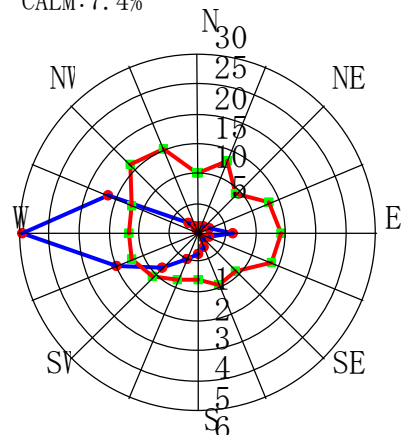
12月 CALM:2.4%
