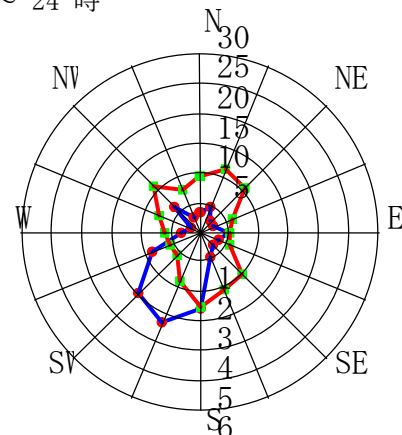
6月 CALM:6.0%
