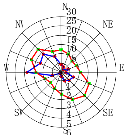
4月 CALM:3.1%
