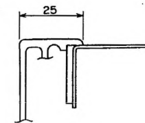
B部詳細 (1/1)
