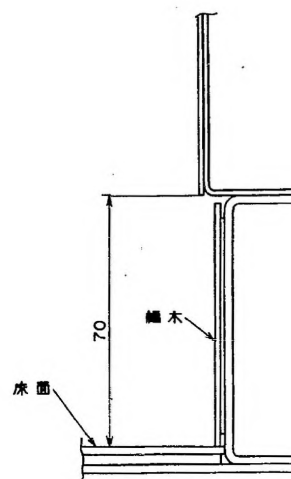
A部詳細 (1/1)
